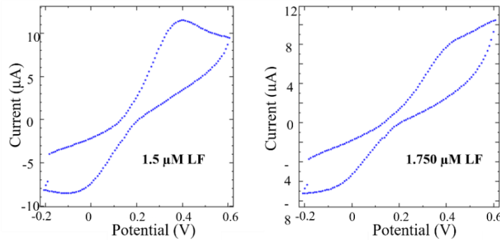
Fig 3. Investigating of increasing lactoferrin concentration using cyclic voltammery curves in the presence of 3 mM [Fe(CN)_6]^{3-/4-} and 0.1 M KCl, potential scan range (-0.2-0.6) volts, scan rate 0.1 V/s, The inset shows a diagram of the corresponding measurement curve.
