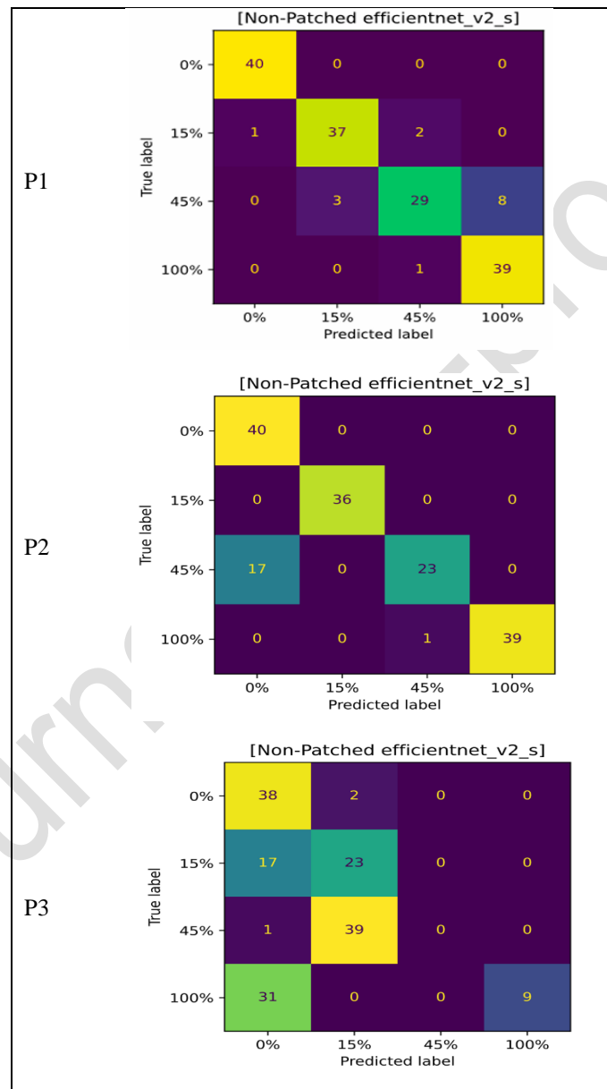
Fig4. Confusion matrix of EfficientNet classifiers in detection of tea adulteration; P1:Tea waste, P2:Foreign Tea, P3, Expired tea
