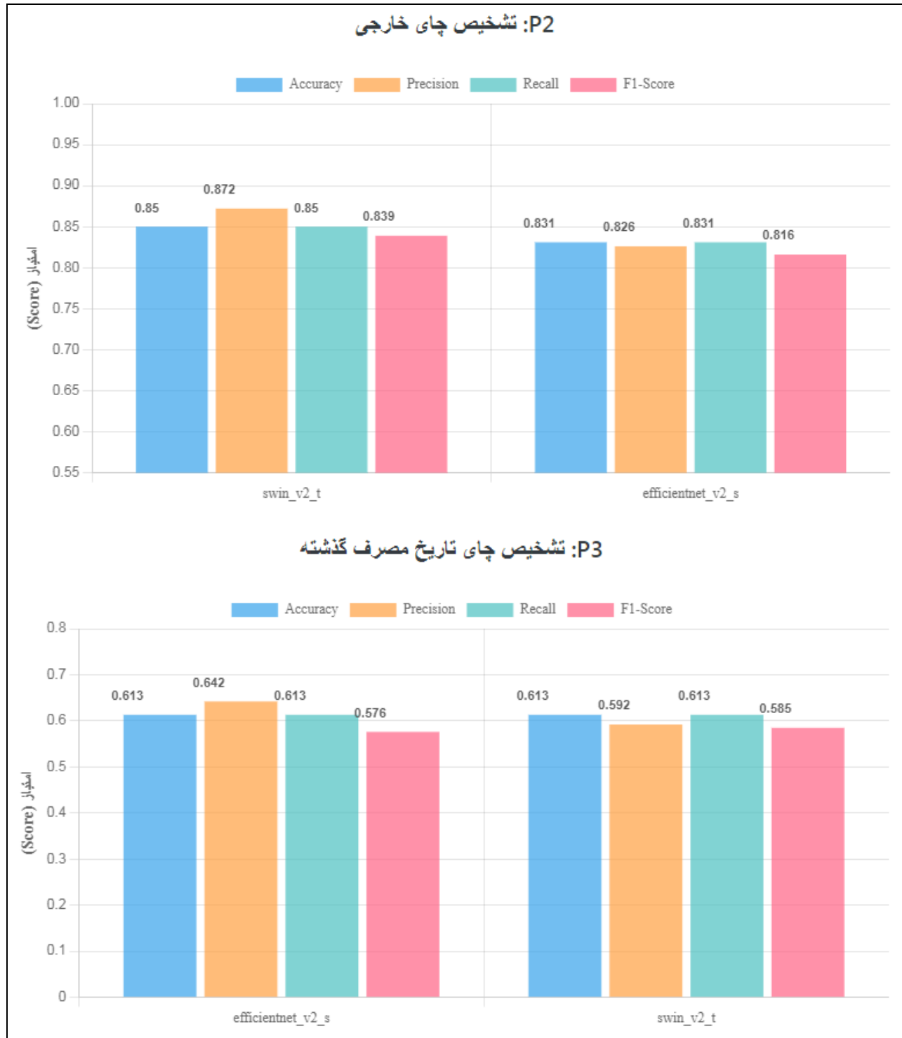
Fig7. Comparison of proposed classifiers from view point of performance criteria in detection of tea adulteration
