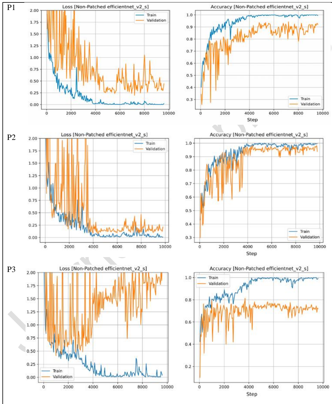
Fig3. Loss-train-validation and accuracy-train-validation of EffecientNet classifiers in detection of tea adulteration; P1:Tea waste, P2:Foreign Tea, P3, Expired tea
