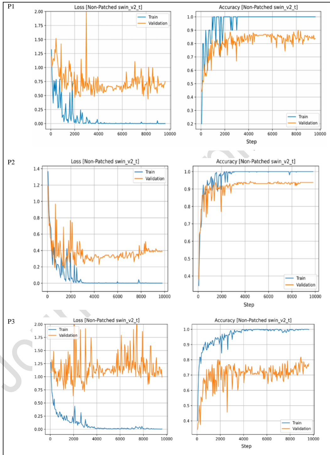
Fig5. Loss-train-validation and accuracy-train-validation of Swin Transform classifiers in detection of tea adulteration; P1:Tea waste, P2:Foreign Tea, P3, Expired tea
