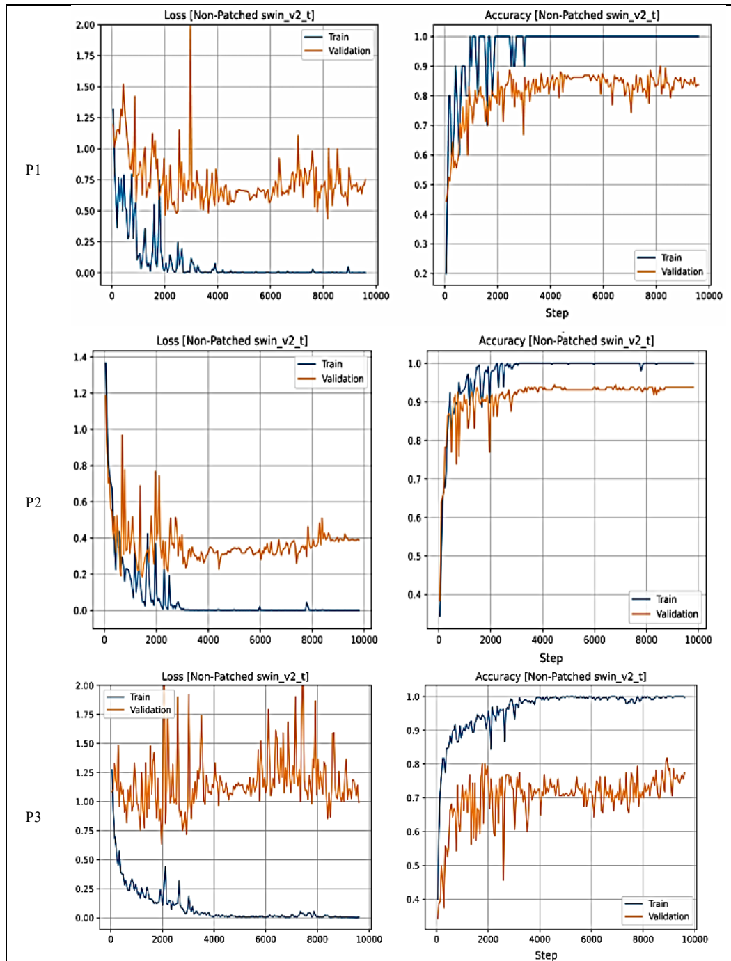
Fig. 5. Loss-train-validation and accuracy-train-validation of Swin Transform classifiers in detection of tea adulteration; P1:Tea waste, P2:Foreign Tea, P3: Expired tea
