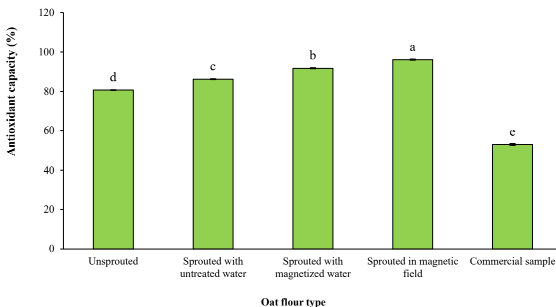
Fig 6. Antioxidant capacity of unsprouted and sprouted oat flours compared to commercial sprouted oat flour. Error bar represents the standard deviation of replicates (n=3). Different letters represent the statistically significant differences at p < 0.05 (Duncan test) between different treatments.
