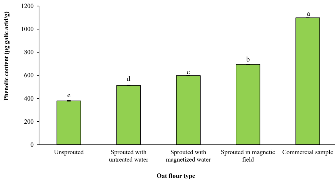
Fig 5. Total phenolic content of unsprouted and sprouted oat flours compared to commercial sprouted oat flour. Error bar represents the standard deviation of replicates (n=3). Different letters represent the statistically significant differences at p < 0.05 (Duncan test) between different treatments.
