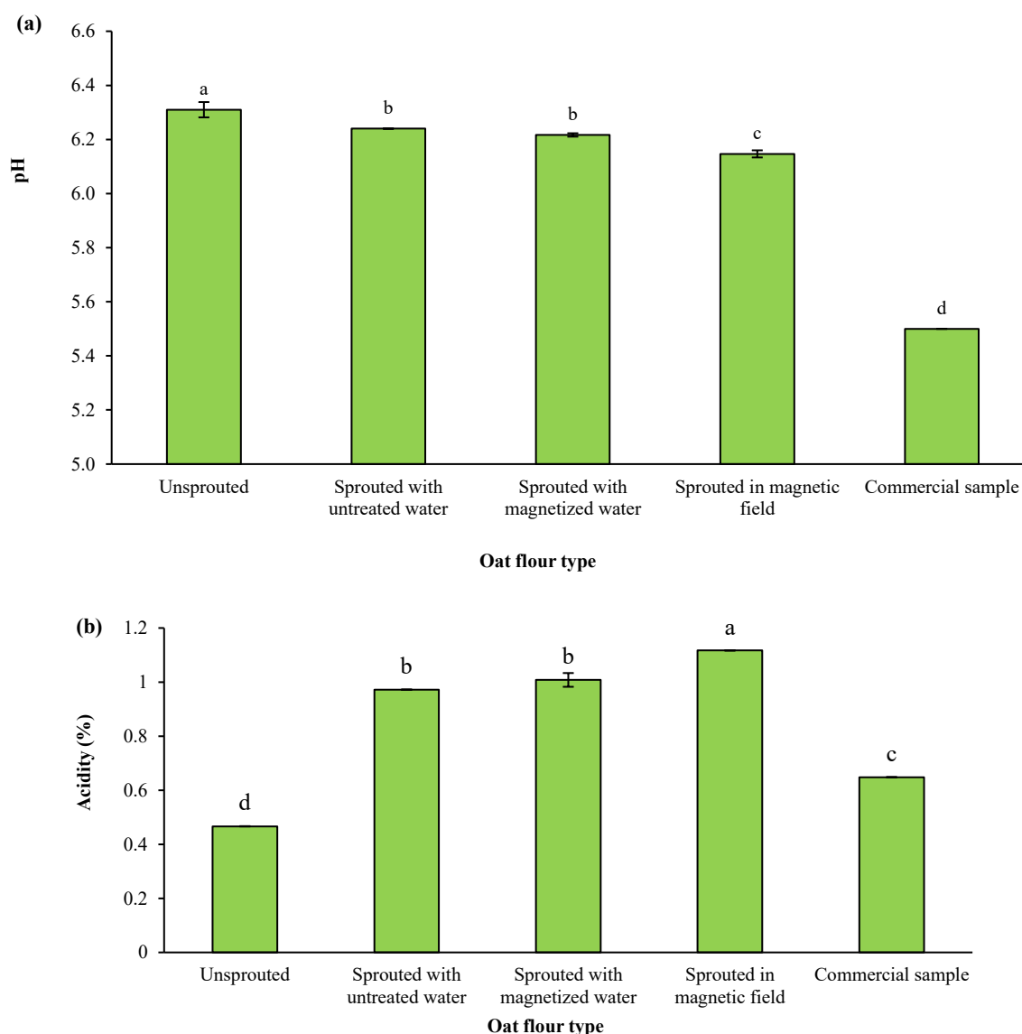
Fig 3. pH (a) and acidity (b) of unsprouted and sprouted oat flours compared to commercial sprouted oat flour. Error bar represents the standard deviation of replicates ( n=3 ). Different letters represent the statistically significant differences at p<0.05 (Duncan test) between different treatments.
